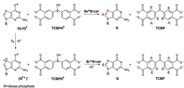
Scheme 2 Protonation of the G(-H)^{\bullet} radical as a source of CIDNP sign change in products of reactions of guanosyl and TCBP radicals. The g -factors of the radicals G(-H)^{\bullet} , TCBP^{\bullet} , and (G^{\bullet+})' are denoted as g_N , g_{TCBP} , and g_C , respectively. A and E denote enhanced absorption and emission of NMR signals for the corresponding protons, respectively.
