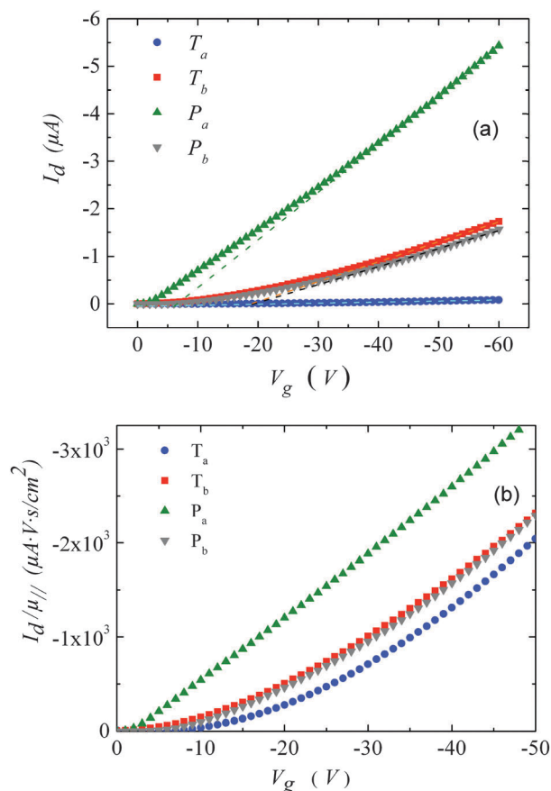
Fig. 3 (a) Transfer characteristics measured at room temperature. (b) Drain current, normalized by the mobility values given in Table 1 versus gate-voltage. The drain voltage was set to -10\text{ V} .
