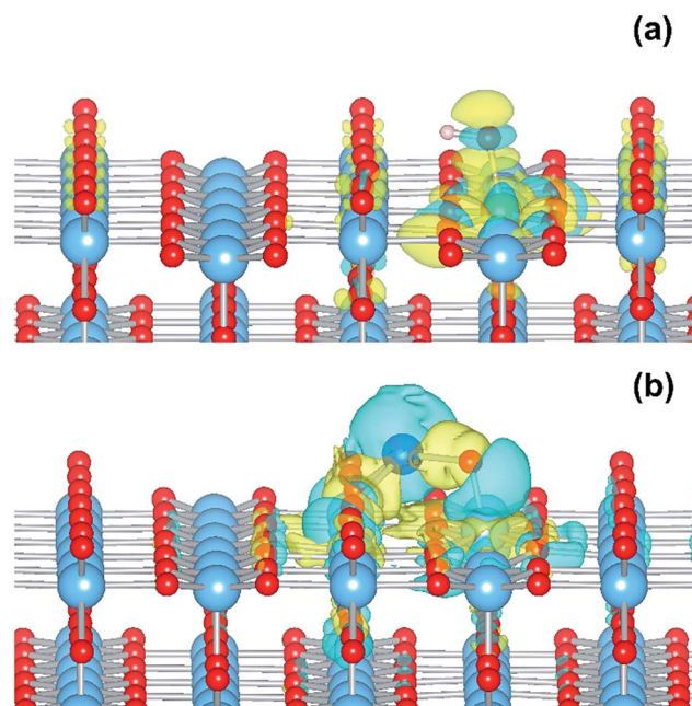
Fig. 9 (a) Charge density difference for the \text{TiO}_2(\text{R})\text{--Fe}(\text{V}_{\text{Ti}}) system upon electron injection and polaron relaxation. (b) Charge density difference for the \text{TiO}_2(\text{R})\text{--Cu} system upon electron injection and polaron relaxation. Blue represents charge density accumulation, yellow charge density depletion.
