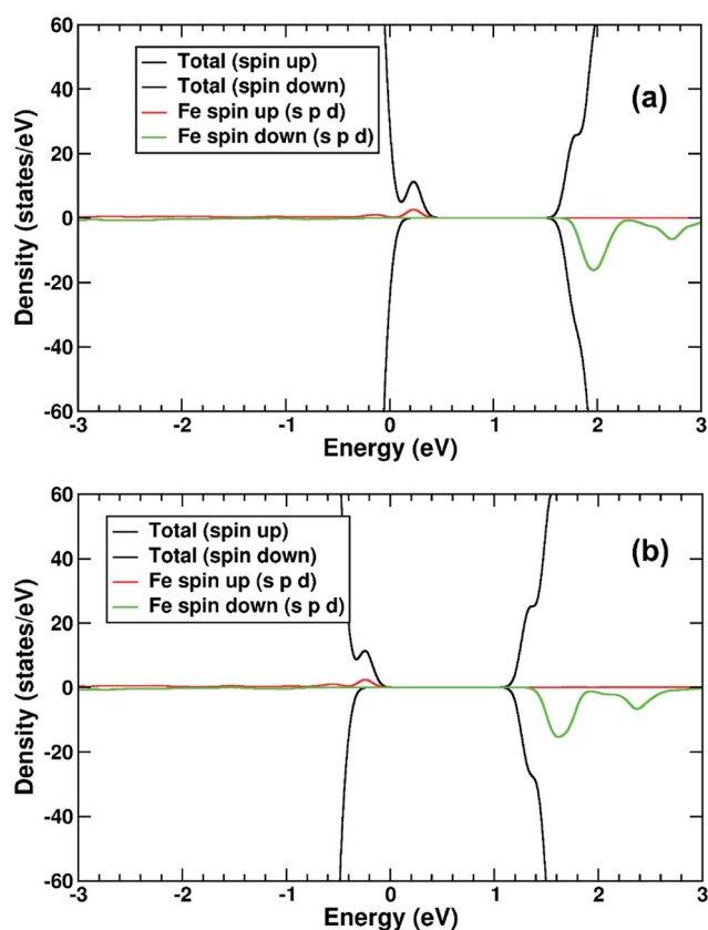
Fig. 8 (a) DOS of \text{TiO}_2(\text{R})\text{--Fe}(\text{V}_{\text{Ti}}) . (b) DOS of the electronic polaron structure of \text{TiO}_2(\text{R})\text{--Fe}(\text{V}_{\text{Ti}}) . The red line represents projection of Fe states in spin up channel, green line projection of Fe states in spin down channel. The zero of the x-axis is set to the top of the VBM.
