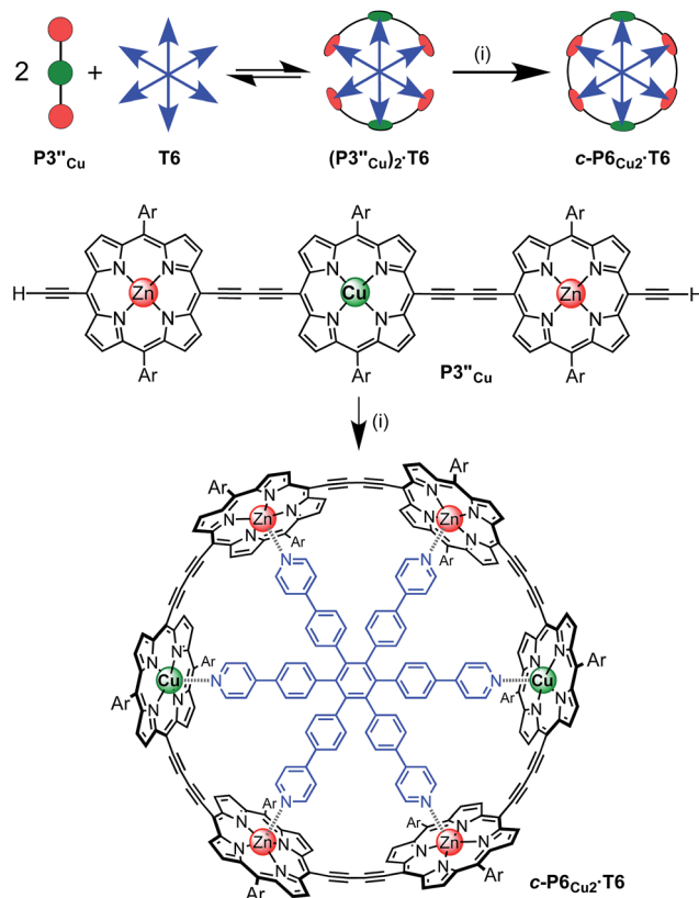
Scheme 2 Synthesis of c-P6 Cu2 ·T6 . Two representations of the synthetic route used to prepare c-P6 Cu2 ·T6 . Reaction conditions: (i) PdCl_2(PPh_3)_2 , CuI , 1,4-benzoquinone, i-Pr_2NH , CHCl_3 , 2%. Ar = 3,5-bis( tert -butyl)phenyl.
