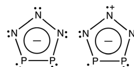
Scheme 1 Schematic depiction of P_2N_3^- and the lowest electronic state ( ^2A_1 ) of P_2N_3^{\cdot-} .
