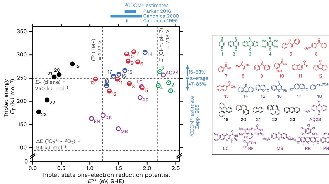
Fig. 8 Triplet energies ( E_T , \text{kJ mol}^{-1} ) vs. triplet state one-electron reduction potentials ( E^{\circ*}({}^3\text{S}^*/\text{S}^-) , V SHE) for a selection of 23 DOM-like model compounds and a selection of widely used sensitizers. The horizontal lines correspond to the triplet excited state energy of a typical diene energy transfer probe and the singlet state energy of \text{O}_2 . The vertical lines correspond to the one-electron oxidation potentials of TMP, E^{\circ}(\text{ArOH}^+/\text{ArOH}) , and hydroxide at pH 7, E^{\circ}(\text{OH}^+/\text{OH}^-) . Selected estimates for {}^3\text{CDOM}^* values from Zepp, 9 Canonica, 79,106 and Parker and Mitch 48 are also shown. The data used for this figure is compiled in Table 1 along with the abbreviation definitions.
