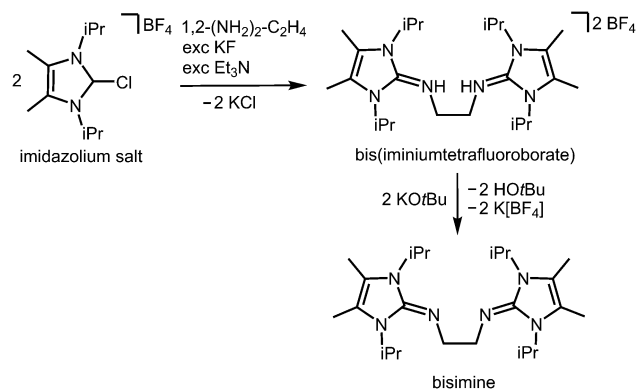
Scheme 15 Synthesis of the bisimine compound 1,2-( L^{iPrMe_2}N )- C_2H_4 ( L^{iPrMe_2} = 1,3 -diisopropyl-4,5-dimethyl-imidazolin-2-ylidene) from an imidazolium salt precursor.
