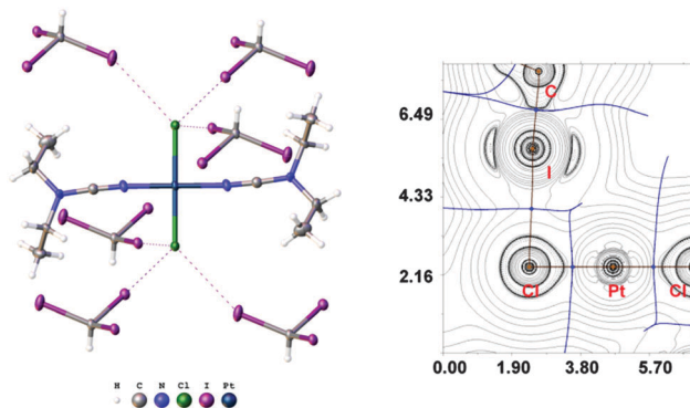
Fig. 4 Left: View of fragment 2 ·(CHI 3 ) 6 from 2 ·2CHI 3 . Thermal ellipsoids are shown with 50% probability and short contacts are indicated by dotted lines. Coordinates of this fragment were applied in further DFT calculations. Right: Contour line diagram of the Laplacian distribution \nabla^2\rho(r) (cross-section along the plane Pt–Cl–I) was received as a result of the topological analysis of the electron density distribution in the model structure. Bond paths are shown as brown lines, selected zero-flux surfaces – as blue lines, bond critical points (3, –1) are shown in blue, nuclear critical points (3, –3) – in pale brown, length unit – Å.
