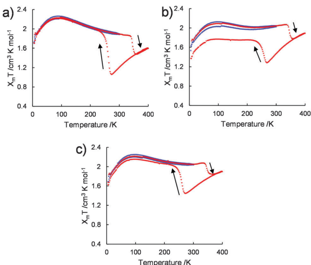
Fig. 4 \chi_m T versus T for (a) 1/[Co^{II}(\text{MeO-terpy})_2] , (b) 2/[Co^{II}(\text{MeO-terpy})_2] and (c) 3/[Co^{II}(\text{MeO-terpy})_2] on warming ( \blacktriangle ) and cooling ( \blacktriangledown ). The blue plots indicate the first cycle (from 5 to 300 \text{ K} ) and the red plots indicate the second cycle above the boiling point of water (from 5 to 400 \text{ K} ).
