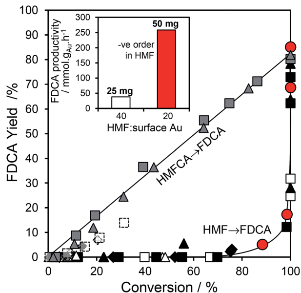
Fig. 5 (main) Disparate evolution of FDCA yield as a function of either HMF or HMFA conversion over 25 mg \triangle(\triangle) 0.5 wt%, \blacklozenge(\blacklozenge) 1 wt%, \square(\square) 2 wt%, \blacksquare(\blacksquare) 5 wt%, and \blacktriangle(\blacktriangle) 10 wt% Au/HT catalysts, and 50 mg \bullet(\bullet) 2 wt% Au/HT; (inset) normalised FDCA productivity per Au atom as a function of HMF : surface Au molar ratio for 2 wt% Au/HT highlighting self-poisoning by high HMF concentrations.
