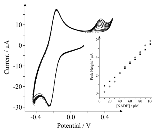
Fig. 4 Cyclic voltammograms obtained utilising an EPPG electrode in pH 7 PBS (with 0.1 M KCl) containing 0.5 mM \text{Ru}(\text{NH}_3)_6^{2+/3+} (internal standard); 'blank' (dotted line) and following successive additions of NADH in the range of 10 to 100 \mu\text{M} (solid lines). Inset : calibration plots of NADH concentration versus the respective voltammetric peak height, obtained using cyclic voltammetry at the EPPG electrode with the internal standard utilised (grey-circles) and without incorporation of the internal standard (black-squares, thus using only pH 7 PBS with 0.1 M KCl as the supporting buffer). All measurements performed at a scan rate of 100 \text{mV s}^{-1} (vs. SCE).
