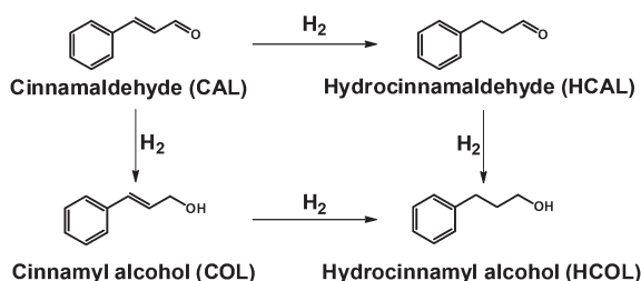
Scheme 2 Reaction paths for the hydrogenation of cinnamaldehyde.
