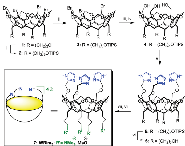
Scheme 2 Synthesis of the tris-imidazole bowl ligand WRim 3 .† (i) TIPSCl, imidazole, DMF, r.t., 82%; (ii) n -BuLi (1 equiv.), THF, -78\text{ }^{\circ}\text{C} , then MeOH -78\text{ }^{\circ}\text{C} \rightarrow \text{r.t.} , 81%; (iii) n -BuLi (3.3 equiv.), THF, -78\text{ }^{\circ}\text{C} , then \text{ClCO}_2\text{Me} , -78\text{ }^{\circ}\text{C} \rightarrow \text{r.t.} ; (iv) \text{LiAlH}_4 , THF, 0\text{ }^{\circ}\text{C} \rightarrow \text{r.t.} , 74% over 2 steps; (v) 2-chloromethyl-1-methyl-1H-imidazole hydrochloride, NaH, DMF, 0\text{ }^{\circ}\text{C} \rightarrow \text{r.t.} , 74%; (vi) TFA, THF– \text{H}_2\text{O} , r.t., 91%; (vii) MsCl, DIPEA, DMF, 0\text{ }^{\circ}\text{C} \rightarrow \text{r.t.} , (viii) \text{NMe}_3 , 40\text{ }^{\circ}\text{C} , 85%.
