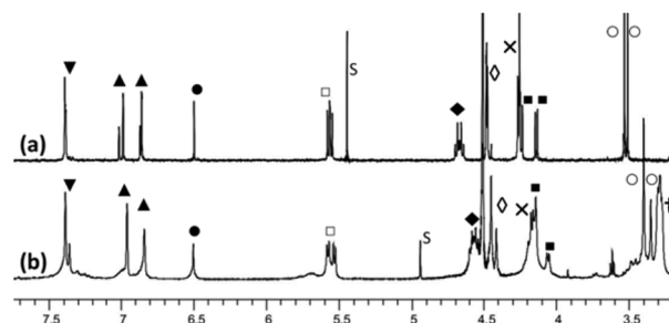
Fig. 1 ^1\text{H} NMR spectra (500 MHz, 300 K) of (a) organosoluble Rim 3 ligand in \text{CD}_3\text{CN} and (b) water-soluble WRim 3 ligand in \text{D}_2\text{O} (2.6 mmol). (▼) HAR. “down”; (▲) HIm; (●) HAR. “up”; (□) and (▢) \text{OCH}_2\text{O} ; (♦) -\text{CHAr} ; (×) \text{CH}_2\text{Im} ; (x) \text{ArCH}_2\text{O} ; (○) \text{NCH}_3 ; (◆) -\text{CHAr} ; (†) \text{CH}_2\text{N}^+\text{Me}_3 . S stands for solvent.
