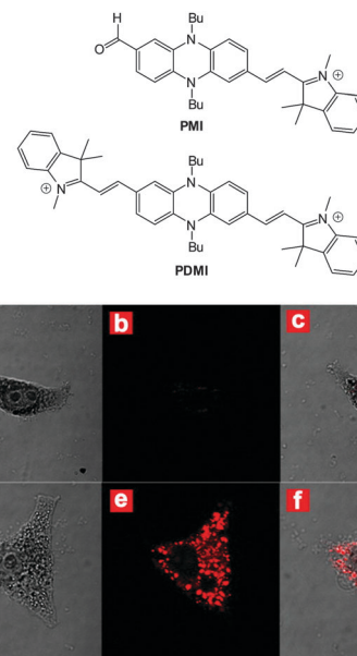
Fig. 32 Top: structures of PMI and PDMI . Bottom: images of HeLa cells incubated with PMI : bright-field (a), dark-field (b) and merged (c). Images of HeLa cells incubated with PMI then \text{CN}^- : bright-field (d), dark-field (e) and merged (f). Image reproduced with permission. 178
