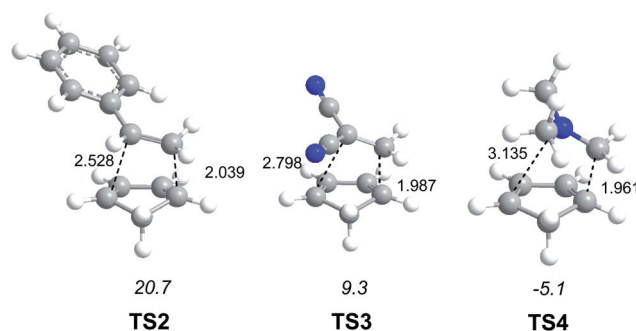
Fig. 2 TSs involved in the DA reactions of Cp 4 with styrene 5 , TS2 , with dicyanoethylene 6 , TS3 , and with iminium cation 7 , TS4 . Relative energies are given in \text{kcal mol}^{-1} , while distances are given in Angstroms.
