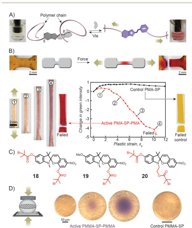
Fig. 11 Spiropyran as a mechanophore. (A) Effect of sonication on the colour of the solution of a spiropyran whose chromene and indoline moieties are functionalised with PMA chains (PMA-SP-PMA; prepared using precursor 18 in (C)). (B) Effect of tensile loading on a dogbone-shaped specimen moulded from a PMA-SP-PMA polymer (bottom left). For comparison, a control sample moulded from a polymer synthesised from a monofunctionalised spiropyran 19 failed without a colour change (bottom right). (C) Structural formulas of precursors of various spiropyran polymers used in the study of mechanoresponsiveness. (D) Colorimetric response of a glassy bead made of PMMA-SP-PMMA to compression (centre). Control bead prepared from a monofunctionalised spiropyran does not change colour upon compression (right). [Adapted with permission from ref. 169 (Copyright 2007 American Chemical Society) (A) and ref. 246 (Copyright 2009 Nature Publishing Group) (B–D).]
