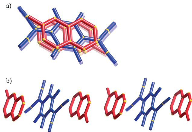
Fig. 6 Stick representations of [(9)_2F_4TCNQ] showing views a) along the stacking direction and b) almost normal to the stacking direction; cations are red, anions are blue.
