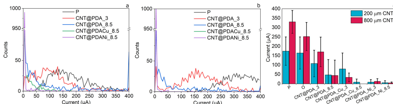
Fig. 5 Distribution of current measured by C-AFM for 200 (a) and 800 (b) \mu\text{m} pristine CTNs, CNTs functionalized with PDA at pH 3 and 8.5, and in the presence of copper and nickel ions. Weighted average current values (c) of 200 and 800 \mu\text{m} pristine and oxidized CNTs, as well as CNTs functionalized with PDA at pH 3 and 8.5, as well as in the presence of copper and nickel ions. Error bars represent the standard deviation from six independent measurements per sample.
