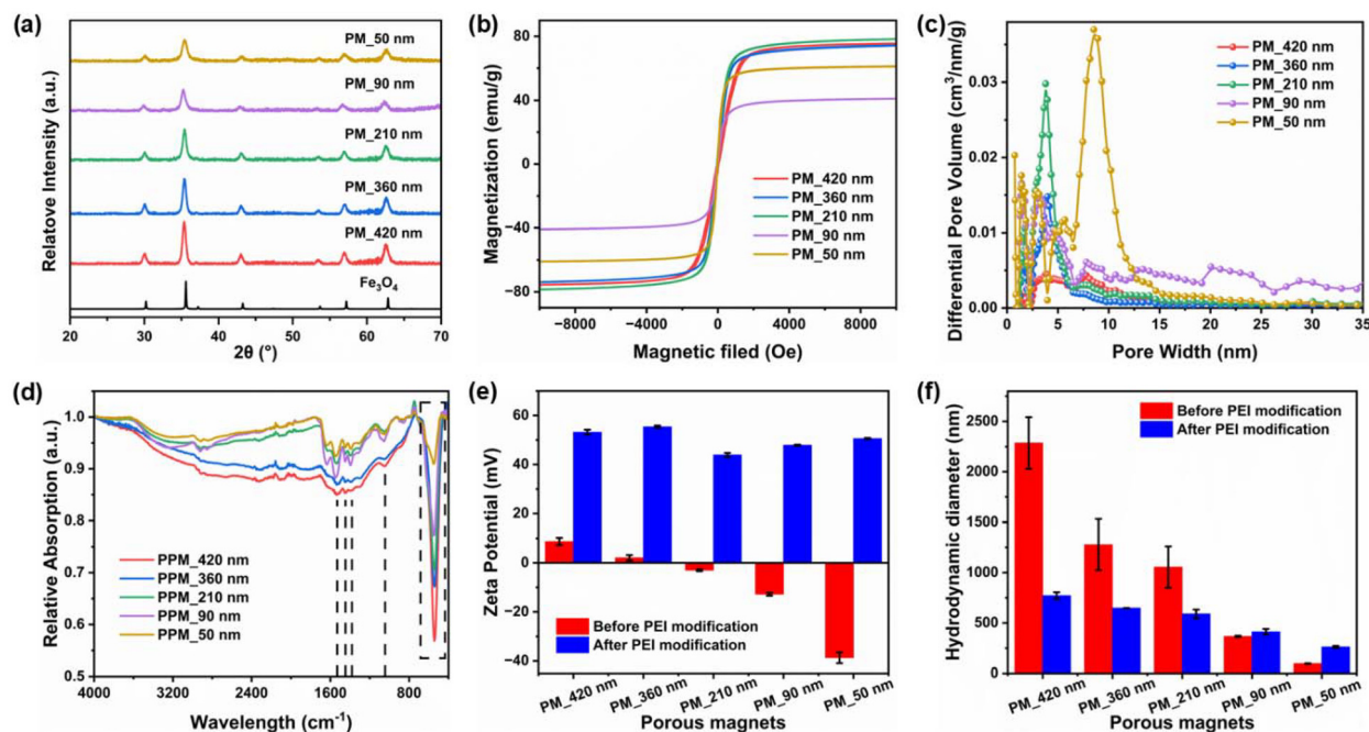
Fig. 2 Characterization of porous magnets before and after PEI modification. The XRD patterns (a), magnetization curves (b) and Non-Local Density Function Theory (NLDFT) slit pore model pore size distribution (c) of porous magnets. The FTIR spectrums of PEI modified porous magnets (d). The zeta potential (e) and hydrodynamic size (f) of porous magnets before and after PEI modification.
