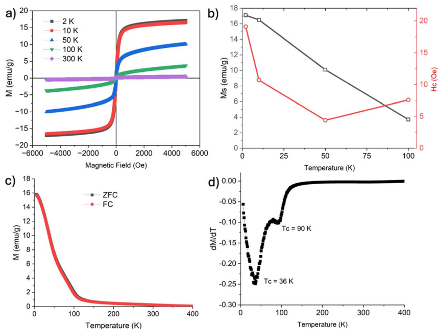
Fig. 7 Magnetic behaviour of the SA750 condition. (a) M-H loops measured at different temperatures, showing ferromagnetic behaviour at low temperatures with decreasing magnetization at higher temperatures. (b) Temperature dependence of saturation magnetization ( M_s , left axis, black squares) and coercivity ( H_c , right axis, red circles). (c) ZFC and FC magnetization curves recorded under a 1000 Oe applied field, showing a gradual decrease in magnetization with increasing temperature. (d) First derivative of magnetization ( dM/dT ), indicating two distinct magnetic transitions with Curie temperatures ( T_c ) at \sim 36 K and \sim 90 K.
