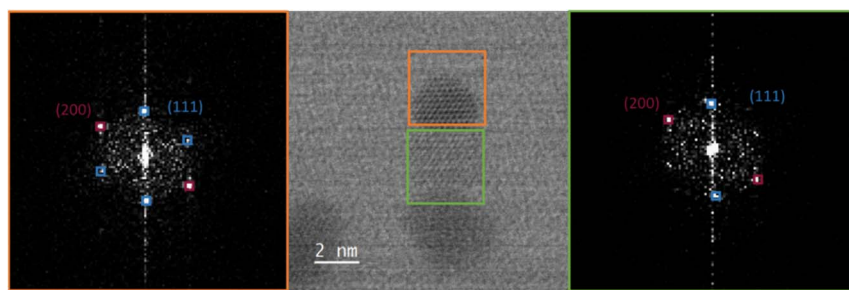
Fig. 5 In the middle, high-resolution STEM image illustrating the epitaxial growth of the Ni_{1-x}Co_xO platelets on the NPs. The FFT images to the left and right of the HR-STEM image are calculated on the NP (orange frame) and on the platelet (green frame), respectively.
