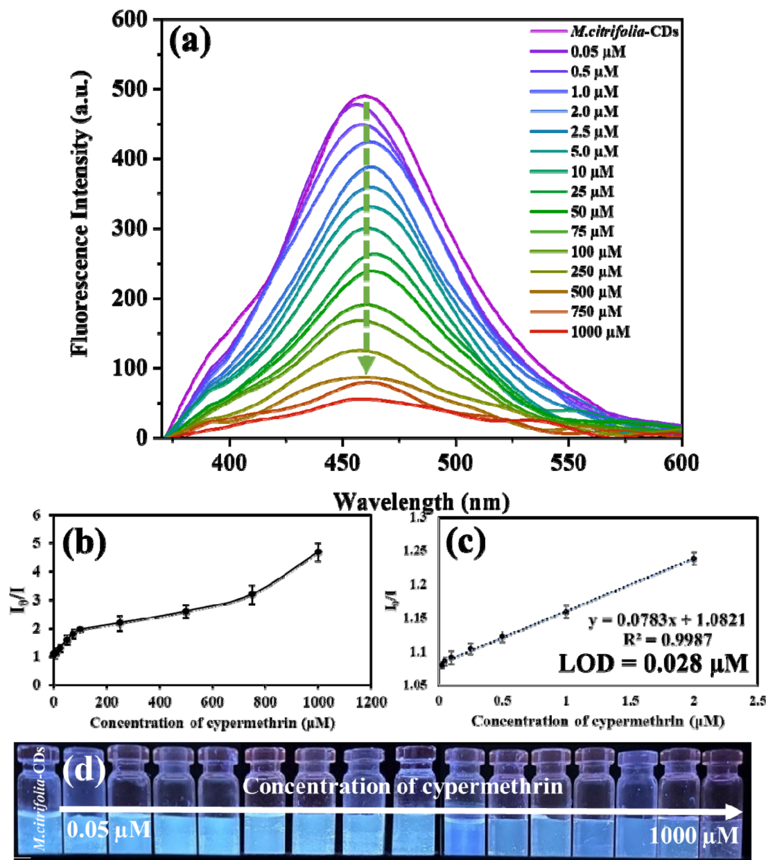
Fig. 7 (a) Fluorescence emission spectra of M. citrifolia -CDs after addition of different concentrations of cypermethrin (0.05–1000 \mu M ) solutions. (b) Stern–Volmer plot between I_0/I and concentrations of cypermethrin. (c) Calibration curve plotted between I_0/I and concentrations of cypermethrin. (d) The photographic representation of fluorescence changes in M. citrifolia -CDs with an increasing concentration of cypermethrin under a UV lamp at 365 nm.
