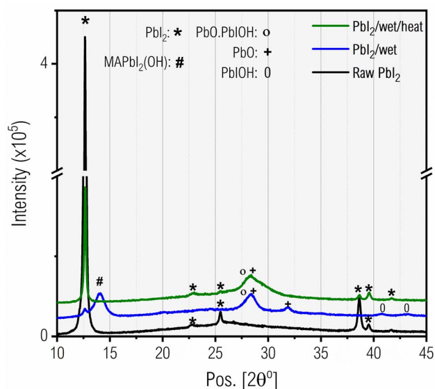
Fig. 5 XRD patterns of Raw- \text{PbI}_2 , \text{PbI}_2/\text{wet} and \text{PbI}_2/\text{wet}/\text{heat} films.
