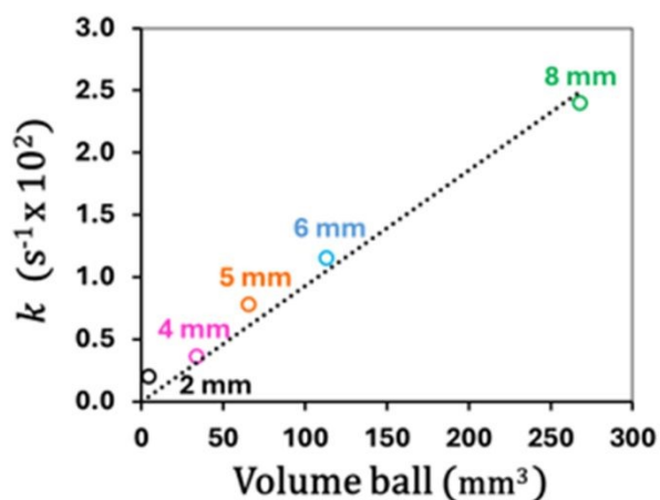
Figure 56 Linear relationship between k , the volume fraction of powder effectively affected by critical loading conditions (CLCs) per unit time, and the milling ball volume (2–8 mm diameter). Data based on kinetic studies outlined in Figure 55. 75 Graph drawn using original data provided by Maria Carta. Adapted from Ref 75 with permission from ACS Sustainable Chemistry & Engineering , 2021, 9, 12591-12601, Copyright {2021} American Chemical Society.
