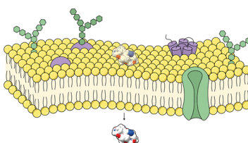
Fig. 4 Chameleonicity and backbone N -methylation as determinants of passive membrane permeability in macrocyclic peptides. Panel (A) Cyclosporin A, a chameleonic molecule, shown in representative open (greater polar surface exposed) and closed (polar surface partially buried) conformations, with electrostatic potential maps (scale in k_B T/e ) that illustrate environment-dependent exposure/burial of polar groups through conformational switching and intramolecular hydrogen bonding. Center: Conceptual schematic of passive diffusion through a lipid bilayer: lower-permeability variants tend to retain solvent-exposed hydrogen-bond donors and acceptors, whereas higher-permeability variants more effectively mask polarity. Panel (B) Parent scaffold cyclo[Leu 1 , D-Leu 2 , Leu 3 , Leu 4 , D-Pro 5 , Tyr 6 ] (compound 1) and the corresponding trimethylated analogue (compound 3), bearing backbone N -methyl groups at D-Leu 2 , Leu 3 , and Tyr 6 (Me)—a modification pattern associated with higher permeability, as reported by White et al. (2011). 93
