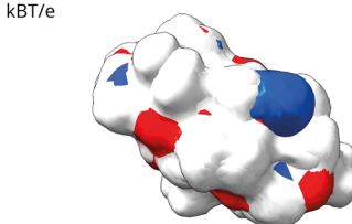
Fig. 4 Chameleonicity and backbone N -methylation as determinants of passive membrane permeability in macrocyclic peptides. Panel (A) Cyclosporin A, a chameleonic molecule, shown in representative open (greater polar surface exposed) and closed (polar surface partially buried) conformations, with electrostatic potential maps (scale in k_B T/e ) that illustrate environment-dependent exposure/burial of polar groups through conformational switching and intramolecular hydrogen bonding. Center: Conceptual schematic of passive diffusion through a lipid bilayer: lower-permeability variants tend to retain solvent-exposed hydrogen-bond donors and acceptors, whereas higher-permeability variants more effectively mask polarity. Panel (B) Parent scaffold cyclo[Leu 1 , D-Leu 2 , Leu 3 , Leu 4 , D-Pro 5 , Tyr 6 ] (compound 1) and the corresponding trimethylated analogue (compound 3), bearing backbone N -methyl groups at D-Leu 2 , Leu 3 , and Tyr 6 (Me)—a modification pattern associated with higher permeability, as reported by White et al. (2011). 93
