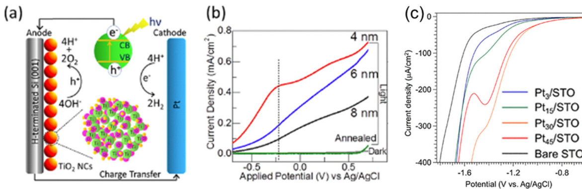
Fig. 7 (a) Schematic diagram of the mechanism of a photoelectrochemical water splitting reaction in the presence of \text{TiO}_2 NC catalysts. An expanded view of a \text{TiO}_2 NC (red spheres at the anode), consisting of Ti (green spheres), O (pink spheres), and H atoms (brown spheres), is shown as the bottom inset. The top inset shows the electron-hole pair generation in \text{TiO}_2 upon UV-vis light illumination, which supplies holes ( h^+ ) for the oxidation of \text{OH}^- leading to \text{O}_2 evolution at the photoanode and electrons ( e^- ), upon traveling to the counter electrode through an external circuit, for reduction leading to \text{H}_2 generation. (b) Photocurrent densities as a function of applied potential obtained in a photoelectrochemical water splitting reaction in a 5 M KOH electrolyte using \text{TiO}_2 NCs of selected sizes (4, 6 and 8 nm) and the post-annealed \text{TiO}_2 NCs (6 nm). The 4 nm NCs show an increased efficiency near -0.25 V, and the overall catalytic performance decreases with increasing size of NCs. Reproduced with permission from ref. 4. Copyright 2014, American Chemical Society. (c) Size-dependent electrocatalytic HER performance with different \text{Pt}_n NCs on STO electrodes in a 0.1 M aqueous solution of \text{Na}_2\text{SO}_4 . The current density of linear sweep voltammetry (LSV) curves from +0.5 V to -1.8 V (vs. Ag/AgCl) provide the hydrogen yield at each voltage. The \text{Pt}_{30} NCs show a discernibly higher (more negative) current density compared to those for both \text{Pt}_{15} and \text{Pt}_{45} . Reproduced with permission from ref. 68. Copyright 2018, Springer Nature.
