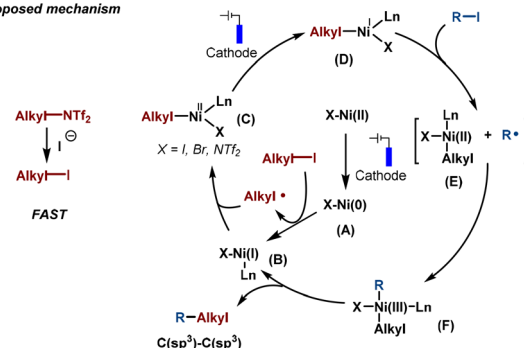
Scheme 24 Proposed mechanism.
