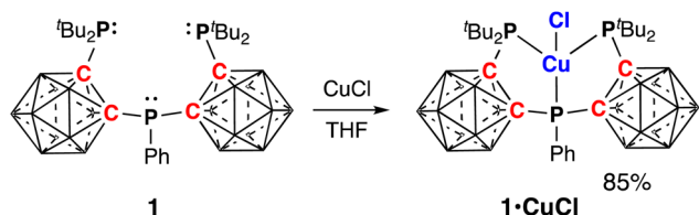
Scheme 3 Synthesis of [ t BuP- closo -(C 2 B 10 ) − PhP- closo -(C 2 B 10 ) − tBuP]CuCl ( 1 ·CuCl). Unlabeled cluster vertices represent BH units.
