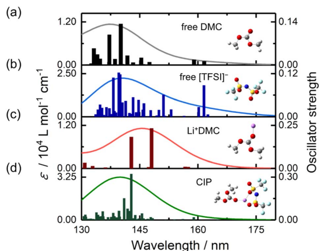
Fig. 4 Theoretical analysis of spectral changes. Time-dependent density functional theory-calculated oscillator strengths and molar extinction coefficients ( \epsilon ) of (a) free DMC, (b) free [\text{TFSI}]^- , (c) \text{Li}^+\text{DMC} and (d) the CIP ( [\text{TFSI}]^-\text{Li}^+\text{DMC} ).
