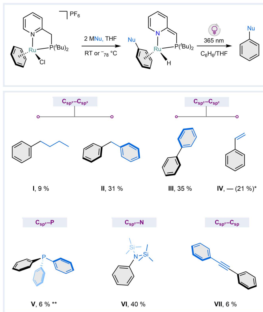
Fig. 6 S N ArH on benzene mediated by complex 1 with various nucleophiles. I: n -butyllithium, II: benzyl potassium, III: phenylmagnesium bromide, IV: vinylmagnesium bromide (quantified based on the qNMR data of the corresponding complex), V: potassium diphenylphosphide (analyzed in the form of its oxide), VI: potassium bis(trimethylsilyl)amide, VII: lithium phenylacetylide (basic work-up was done instead of the UV irradiation). The yields were determined by GC analysis. * based on spectroscopic yield of the corresponding hydride complex; ** based on GC yield of O=PPh 3 following a reaction with H 2 O 2 ; for more details, see ESI Section S4.2.†
