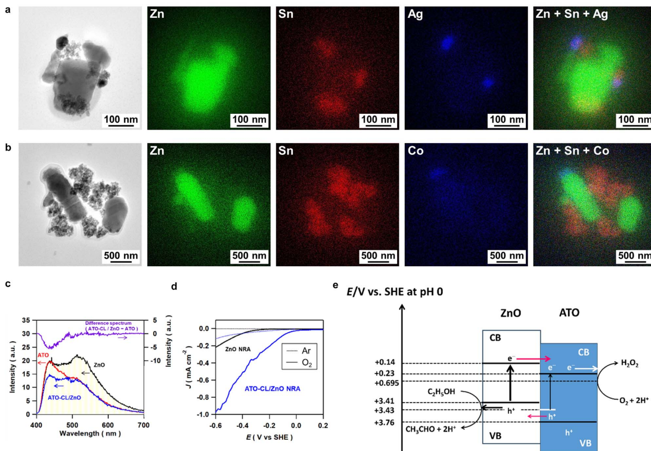
Fig. 3 (a) TEM-EDS elemental mapping of Ag-photodeposited ht-ATO-CL(20)/ZnO(10). (b) TEM-EDS elemental mapping of CoO x -photo-deposited ht-ATO-CL(20)/ZnO(10). (c) PL spectra of ATO, ZnO, and ATO-CL(100)/ZnO(50) NPs on excitation by light with wavelength of 365 nm at 77 K. (d) Dark current ( J )-potential ( E ) curves of ZnO NRA and ATO-CL/ZnO NRA electrodes in argon gas (dotted lines) and oxygen gas (solid lines)-bubbled 0.1 M NaClO 4 electrolyte solution containing 4 vol% ethanol. (e) A reaction mechanism proposed for the present ATO-CL/ZnO-photocatalyzed H 2 O 2 production.
