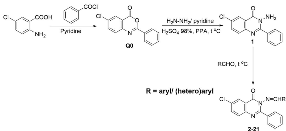
Scheme 1 Synthesis of 3-methylenamino-4(3 H )-quinazolone derivatives (PPA: polyphosphoric acid).
