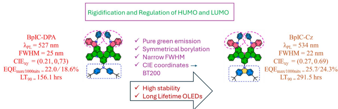
Fig. 78 The molecular structures of green emissive B/N type MR emitters and designed polycyclo-heteraboron MR-TADF materials BpIC-DPA and BpIC-Cz.
