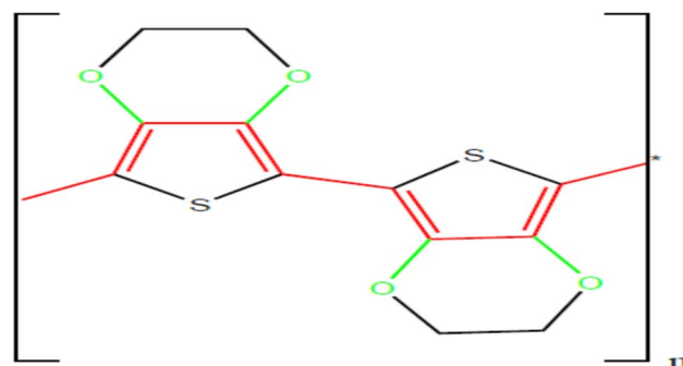
Fig. 17 Chemical structure of conjugated conductive polymer poly(3,4-ethylene dioxathiophene). 163
