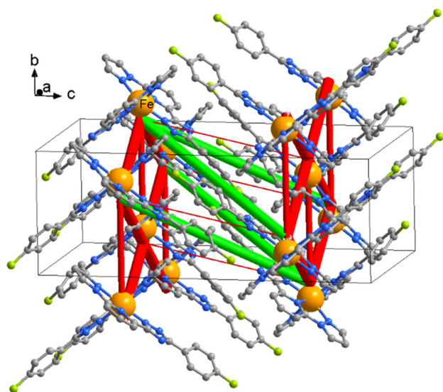
Fig. 8 A fragment of the crystal packing of 4Cl in the HS state superimposed on the differential energy framework, constructed using the values from the Table S5,† column " \Delta E(\text{total})/(\text{HS} - \text{LS}) ", showing negative intra-layer energetics (red cylinders) and positive inter-layer energetics (green cylinders) due to the lattice changes during the ST event. Cylinder thickness is proportional to the absolute value of the interaction energy.
