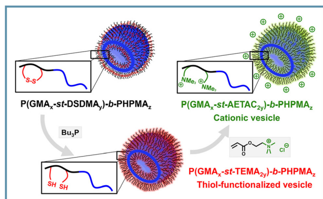
Fig. 3 Schematic illustration of surface-functionalized PISA vesicles based on disulfide cleavage of P(\text{GMA}_x\text{-st-DSDMA}_y)\text{-}b\text{-PHPMA}_z . Adapted with permission from ref. 68. Copyright 2012 American Chemical Society.
