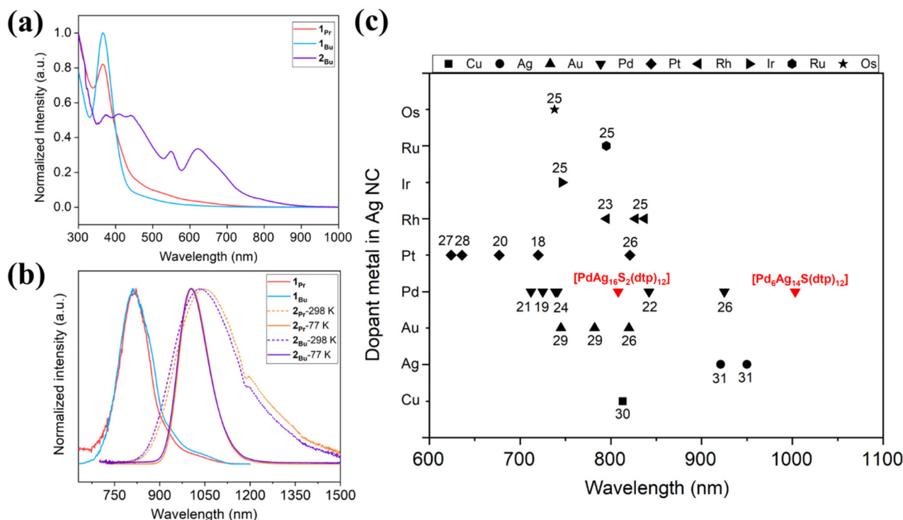
Fig. 3 (a) The absorption spectra for 1_{\text{Pr}} , 1_{\text{Bu}} , and 2_{\text{Bu}} recorded in 2-MeTHF. (b) Emission spectra for 1_{\text{Pr}} ( \lambda_{\text{em}} = 808 nm), 1_{\text{Bu}} ( \lambda_{\text{em}} = 811 nm), 2_{\text{Pr}} ( \lambda_{\text{em}} = 1007 nm) and 2_{\text{Bu}} ( \lambda_{\text{em}} = 1004 nm) in 2-MeTHF at 77 K. (c) Comparison of \lambda_{\text{em}} for doped silver rich NC with entries labeled by the corresponding references.
