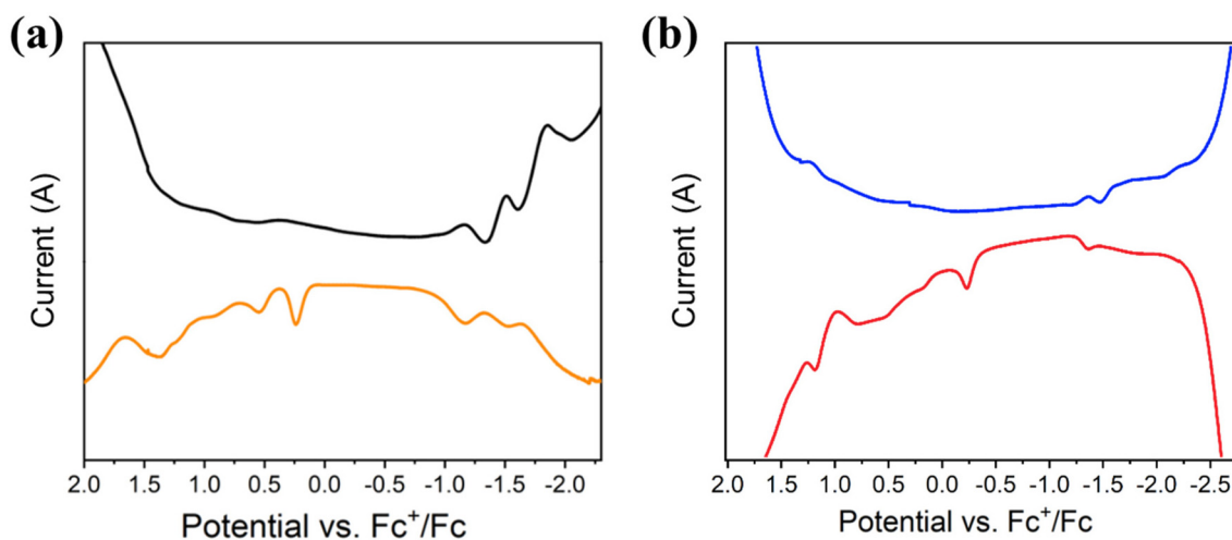
Fig. 4 Square wave voltammetry of 1 Pr , (a) and 2 Bu , (b) recorded in THF and CH 2 Cl 2 , at 298 K containing 0.1 M [ n BuN][PF 6 ] under a N 2 atmosphere.
