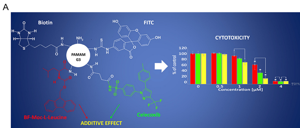
Fig. 24 The structure of compound 33. Schematic formulae of studied conjugates: G3 1B31C (a = 1, b = 31, c = 0, d = 0, e = 0); G3 1B31L (a = 1, c = 31, b = 0, d = 0, e = 0); G3 1B16C15L (a = 1, b = 16, c = 15, d = 0, e = 0); G3 1B20C1F (a = 1, b = 20, c = 0, d = 1, e = 10); G3 1B20L1F (a = 1, b = 0, c = 20, d = 1, e = 10); G3 1B10C10LF (a = 1, b = 10, c = 10, d = 1, e = 10). (A) Drugs and their effects on cell viability. Reproduced with permission. 99 Copyright 2018, Elsevier.
