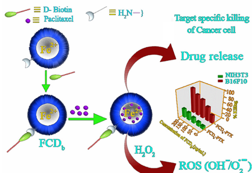
Fig. 44 The structure of compound 60. (A) A picture showing PTX-loaded FCD 6 as a therapeutic agent. Reproduced with permission. 140 Copyright 2021, ACS.
