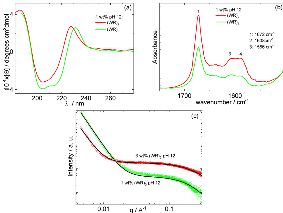
Fig. 6 (a) CD, (b) FTIR and (c) SAXS data for 1 or 3 wt% (WR) n - 2-3 at pH 12. The solid lines in (c) are the fitting of the SAXS data as described in the manuscript. To reduce noise in the data, SAXS data was measured at 3 wt% for (WR) 2 .
