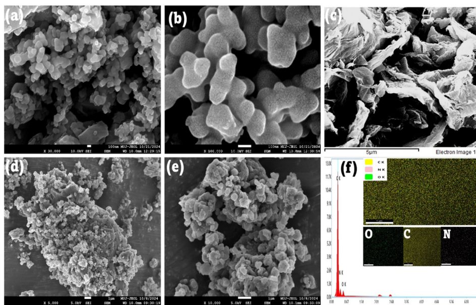
Fig. 4 FESEM images of (a) and (b) PIn, (c) GO and (d) and (e) 15%GO/PIn. (f) EDAX spectrum and color mapping of the 15%GO/PIn composite.
