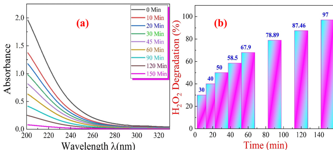
Fig. 28 (a) The UV spectra of the H_2O_2 solutions in the presence of green synthesized CFO nanoparticles. (b) Plot of the percentage of H_2O_2 decomposition versus time in the presence of the prepared CFO at room temperature.
