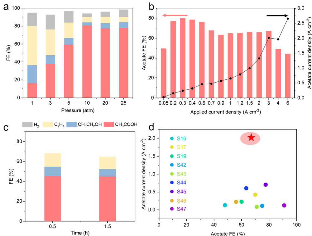
Fig. 4 CORR performance of different cathode electrodes in a flow cell. (a) FEs for various products of \text{Cu}_2(\text{OH})_3\text{Br} at -0.64 \text{ V} versus RHE under different pressures. (b) FEs for various products as a function of total current over \text{Cu}_2(\text{OH})_3\text{Br} . (c) FEs for various products of annealed GBs-Cu (annealing temperature = 300^\circ\text{C} ). (d) Comparison of the catalytic performance of \text{Cu}_2(\text{OH})_3\text{Br} with those recently reported outstanding Cu-based catalysts. 16,17,19,42–47
