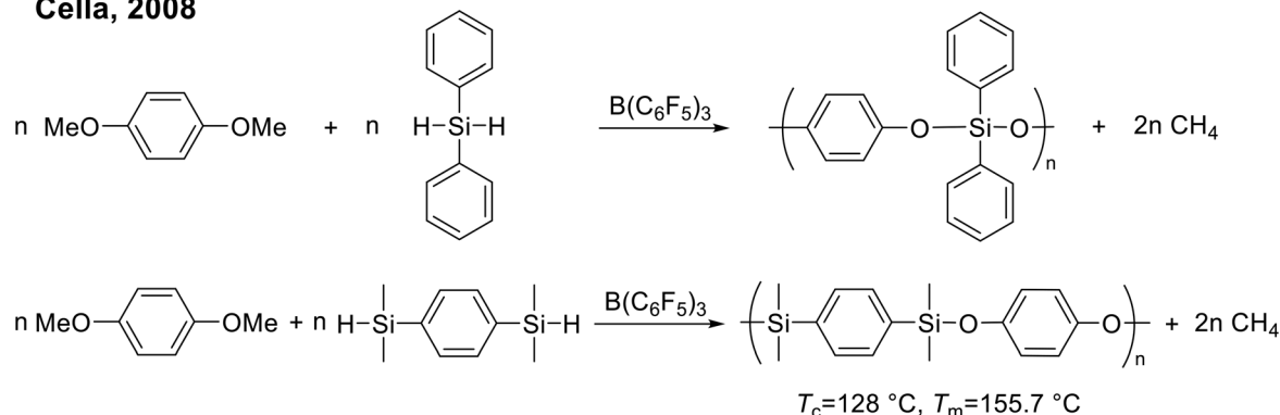
Fig. 8 Polycondensation of a bis(methyl ether) and Ph 2 SiH 2 or BDMSB. 31
