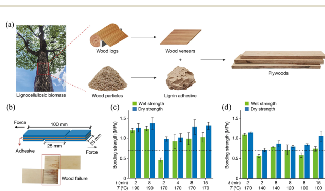
Fig. 9 (a) Schematic illustration of the preparation of plywood from wood veneers with lignin as adhesives. (b) Schematic illustration of three-layer formaldehyde-protected lignin (FPL)-bonded plywood specimens used for adhesion performance tests (top) and wood failure of the specimen after a wet strength test (bottom). (c) Effects of hot-pressing temperatures and times on the adhesion performance of FPL adhesives. (d) The promotion effect of acid addition on the adhesion performances of FPL adhesives. 133 [Reproduced from ref. 133 with permission from Springer Nature, copyright of 2023.]
