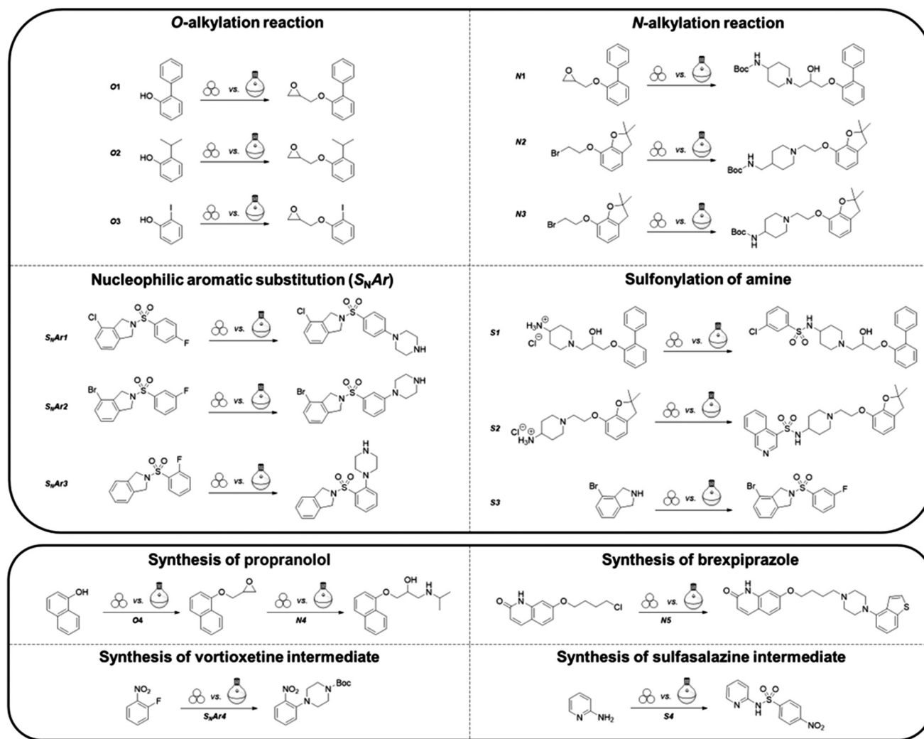
Fig. 5 Selected reactions for verifying the greenness and whiteness of the mechanochemical and solvent-based methods using the RGBsynt model. Experimental conditions for the presented mechanochemical O-alkylation (O1–3), N-alkylation (N1–3), nucleophile aromatic substitutions (S N Ar1–3), and sulfonylation (S1–3) reactions were taken from our previously reported data. 9,22,23 Newly developed synthetic procedures for obtaining selected drugs – propranolol and brexipiprazole as well as intermediates of vortioxetine and sulfasalazine – are presented in detail in the ESI.† Solvent-based chemical transformations are in accordance with in-house protocols, 23–26 and the literature data. 27–31
