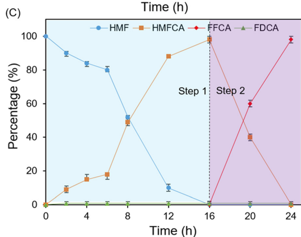
Fig. 2 The chemoenzymatic cascade system for selectively catalyzing the oxidation of HMF to FFCA. (A and C) One-pot two-step method. Reaction conditions: 0.1 mM \text{NAD}^+ , 0.02 mM NFCM, 10 mM HMF, 0.08 \mu\text{M} HLADH, 0.1 \mu\text{M} rAaeUPO and 1 \mu\text{M} GOase were added into 1 mL of phosphate buffer (50 mM, pH 7.0) in turn and shaken at 30 °C (300 rpm). (B) One-pot one-step method. The detection methods of each compound were the same as those in Table 1. Percentage (%) is the ratio of the concentration of each component in the mixture and calculated according to the formula given in section 1.8 in the ESI.†
