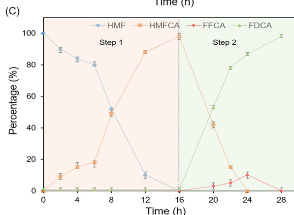
Fig. 3 The selective synthesis of FDCA from HMF. (A and C) One-pot two-step method. Reaction conditions: 0.1 mM \text{NAD}^+ , 0.02 mM NFCM, 10 mM HMF, 0.08 \mu\text{M} HLADH, 0.1 \mu\text{M} rAaeUPO and 1 \mu\text{M} GOase were added into 1 mL of phosphate buffer (50 mM, pH 7.0) in turn and shaken at 30 °C (300 rpm). (B) The oxidation of FFCA to FDCA catalyzed by different chemoenzymatic systems. Reaction conditions and detection methods were the same as those in Table 1. Percentage (%) is the ratio of the concentration of each component in the mixture and calculated according to the formula given in section 1.8 in the ESI.†
