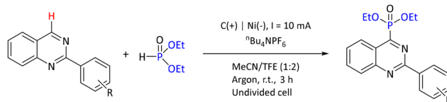
Scheme 30 Electrochemical synthesis of phosphonates.
