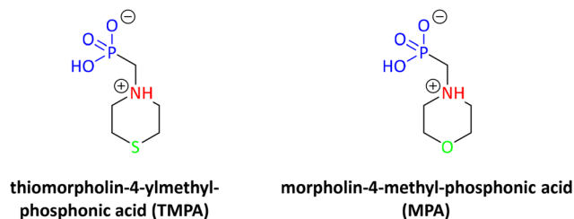
Fig. 26 Schematic structures of the corrosion inhibitors thiomorpholin-4-ylmethyl-phosphonic acid (TMPA) and morpholin-4-methyl-phosphonic acid (MPA).
