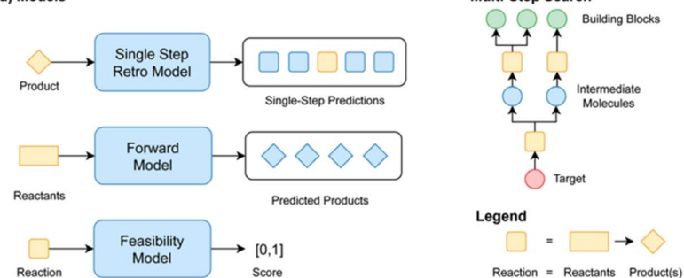
Fig. 15 Benchmarking workflows and metrics for retrosynthesis algorithms in Synthesius, reproduced from https://doi.org/10.1039/d4fd00093e .
