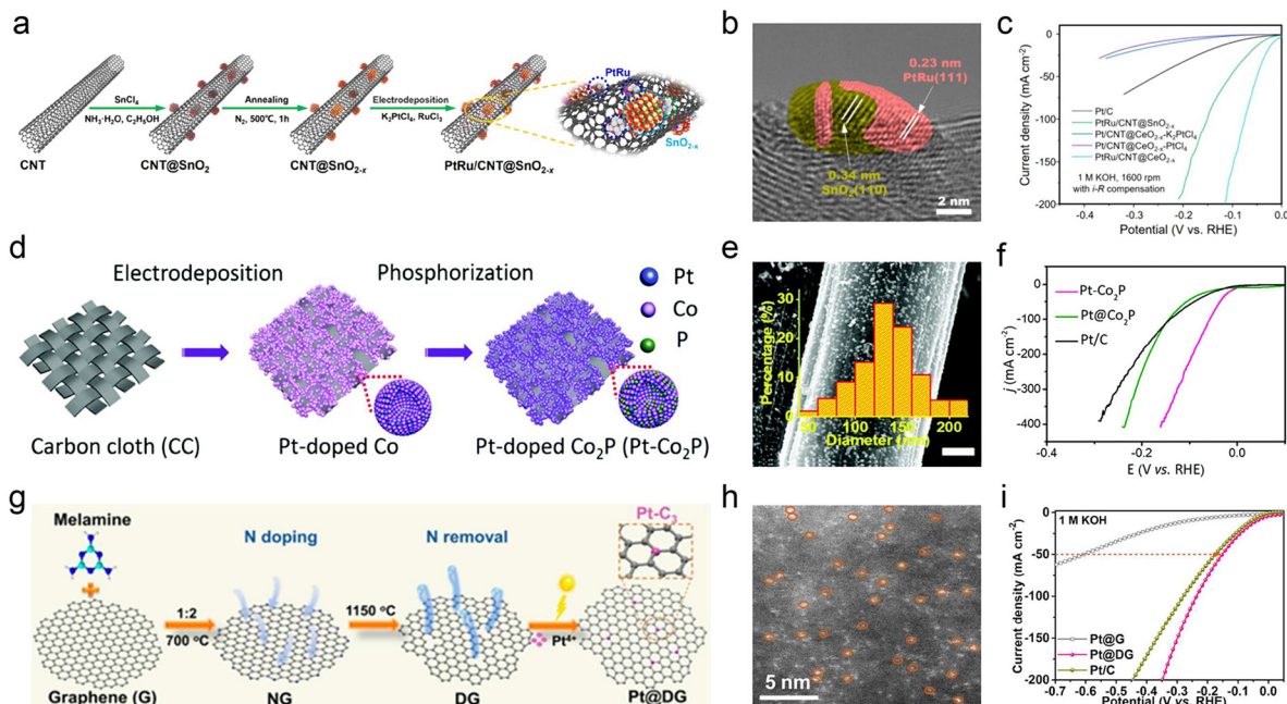
Fig. 7 (a) Schematic diagram of the preparation process of the M/\text{CNT}@SnO_{2-x} catalyst. (b) HRTEM image of \text{PtRu}/\text{CNT}@SnO_{2-x} . The yellow marked area belongs to the SnO_{2-x} nanoparticle, and the pink area represents the electrodeposited Pt and Ru. (c) HER polarization curves for commercial Pt/C, \text{Pt}/\text{CNT}@SnO_{2-x}-K_2PtCl_4 , \text{Pt}/\text{CNT}@SnO_{2-x}-PtCl_4 , and \text{PtRu}/\text{CNT}@SnO_{2-x} in 1 M KOH solution at a scan rate of 10 \text{ mV s}^{-1} . Reproduced with permission. 130 Copyright 2024, American Chemical Society. (d) Schematic illustration of the fabrication process of \text{Pt-Co}_2\text{P} . (e) SEM image of \text{Pt-Co}_2\text{P} particles grown on CC. The inset is the particle size distribution. Scale bar: 2 \mu\text{m} . (f) LSV curves of the catalysts tested at 5 \text{ mV s}^{-1} . Reproduced with permission. 131 Copyright 2020, The Royal Society of Chemistry. (g) Schematic illustration of the preparation of \text{Pt}@DG . (h) HAADF-STEM image of \text{Pt}@DG . (i) Polarization curves of \text{Pt}@G , \text{Pt}@DG , and \text{Pt}/C with a scan rate of 10 \text{ mV s}^{-1} . Reproduced with permission. 132 Copyright 2022, American Chemical Society.
