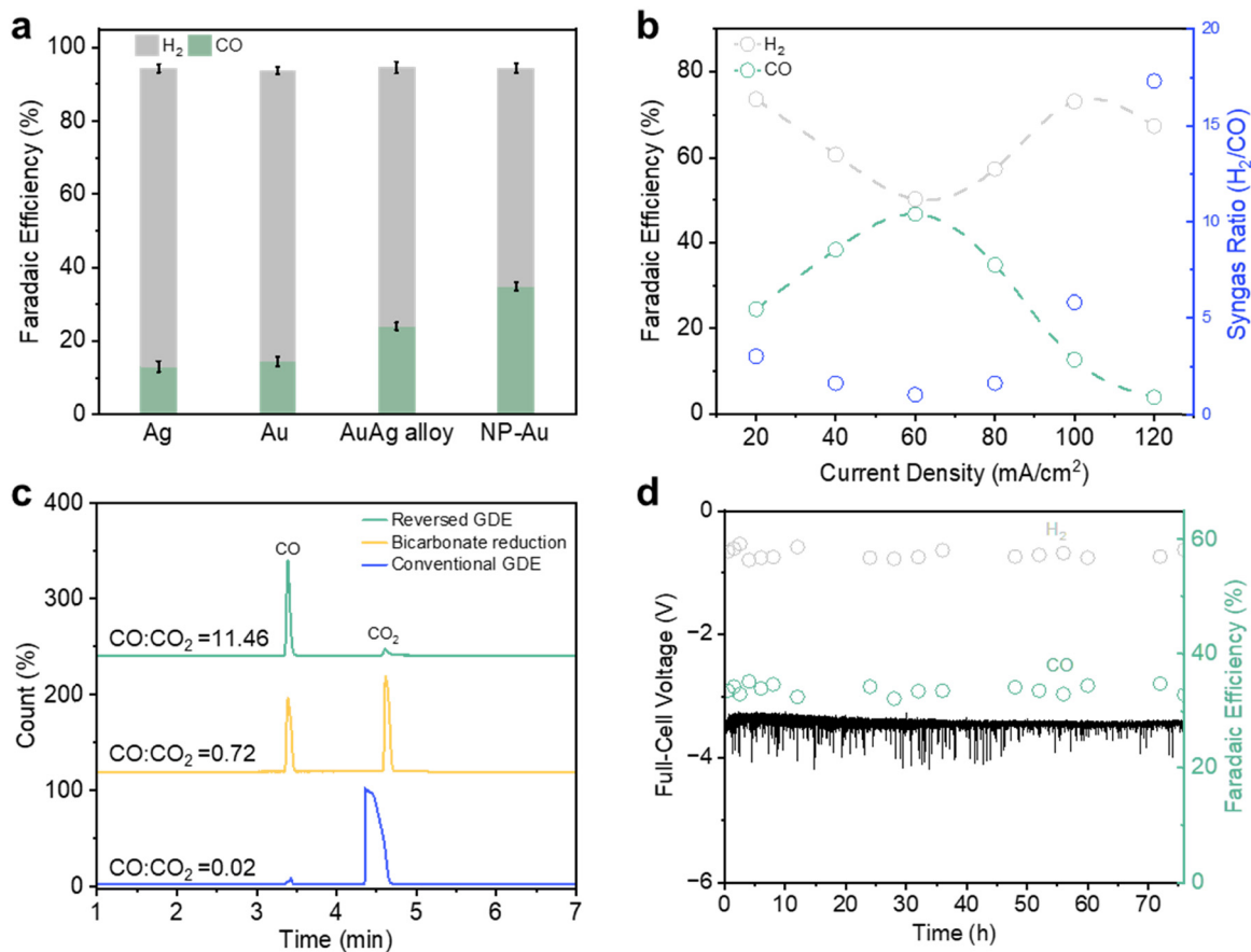
Fig. 5 High purity syngas production and collection. (a) Product FE to \text{H}_2 and CO for the different catalysts at 80 \text{ mA cm}^{-2} using PTFE with a pore size 0.45 \mu\text{m} as the GDL. (b) Product FE with NP Au/PTFE as catalyst at different current densities. (c) GCMS data of the gas product collected using different cell configurations with a current density of 80 \text{ mA cm}^{-2} , without using \text{N}_2 as the carrier gas for the reversed GDE case. Note: conventional GDE uses a continuous 30 \text{ sccm CO}_2 flow rate. The ratios displayed are calculated based on the area of the CO and \text{CO}_2 peaks in the GCMS data. (d) Long term operation of NP-Au at 80 \text{ mA cm}^{-2} in the reversed GDE mode over a 76 h testing period.
